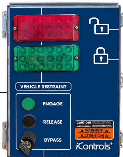
Vehicle Restraint Panel with Stop and Go LED Light Display
